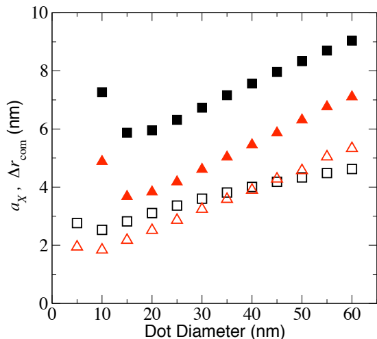
FIG. 4: (Color online) Exciton radius a_X ( \square 's) and exciton center of mass fluctuations \Delta r_{\text{com}} ( \triangle 's) for InGaAs/GaAs dots with a 6 ML wetting layer (full symbols) and for CdSe/ZnSe dots (open symbols).
