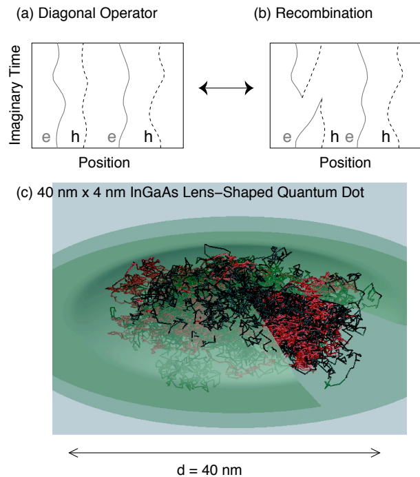
FIG. 1: (Color online) Illustration of our path-integral calculation of biexciton recombination rates in self-assembled quantum dots. We express the rate as a ratio of path integrals with (a) diagonal and (b) radiating constraints, see Eq. (6). We evaluate the path integrals using Monte Carlo integration on realistic three-dimensional models. A typical path contributing to the integrals for an InGaAs/GaAs dot is shown in (c). These paths sample the probability density, energy, rate, and other properties of the radiating states.
